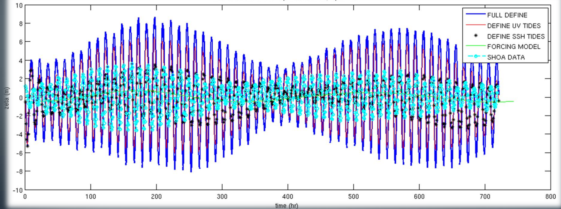
ROMS sea level anomaly. Puerto Montt, April 1993
