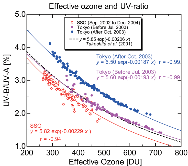
Figure 3 – UV-ratio (UV-B/UV-A) of spectroradiometer with respect to effective ozone. For SSO data (○, red), ozone data of SSO with Brewer spectrometer was used. For Tokyo (●, violet and blue), ozone data of Tsukuba was used. Data points clearly separated into two parts due to replacement of spectroradiometer. Least square fitting results are shown as solid lines. Dashed line indicates function of Takeshita et al. (2001).
